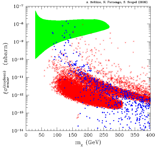
Figure 3. Scatter plot of the values of the product \xi \sigma_{\text{scalar}}^{(\text{nucleon})} between the scaling parameter \xi and the neutralino–nucleon scalar cross section, vs. the neutralino mass m_\chi , for a generic scan of the mSUGRA parameter space. (Red) crosses refer to 0.05 \leq \Omega_\chi h^2 \leq 0.3 , while (blue) dots denote configurations with \Omega_\chi h^2 < 0.05 . m_b , m_t and \alpha_s are varied inside their 95% C.L. allowed ranges. The shaded (green) area [7] shows the region which, for a relic particle with pure coherent interactions, is compatible with the annual modulation effect observed by the DAMA/NaI experiment [8].
